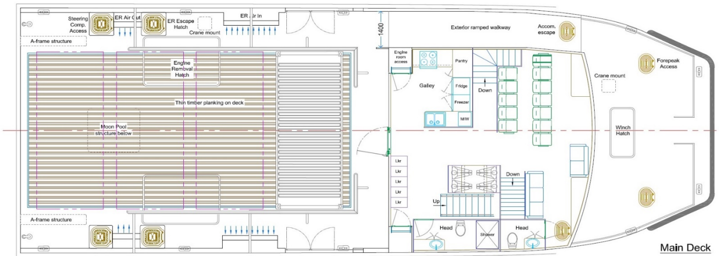
Deck Arrangement with 20' Containers
