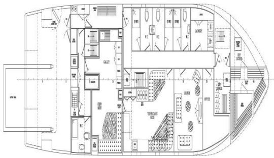
MAIN DECK
